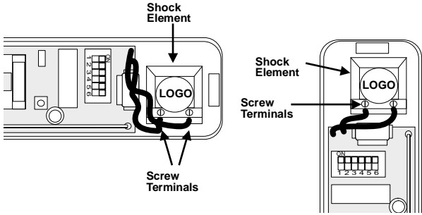
Figure 3. Positioning shock element according to mounting orientation on a vertical surface
